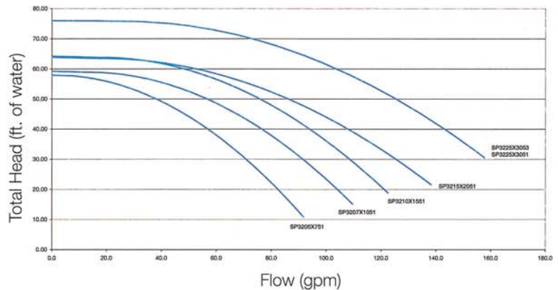
TriStar, 50 Hz Flow vs. Total Head
