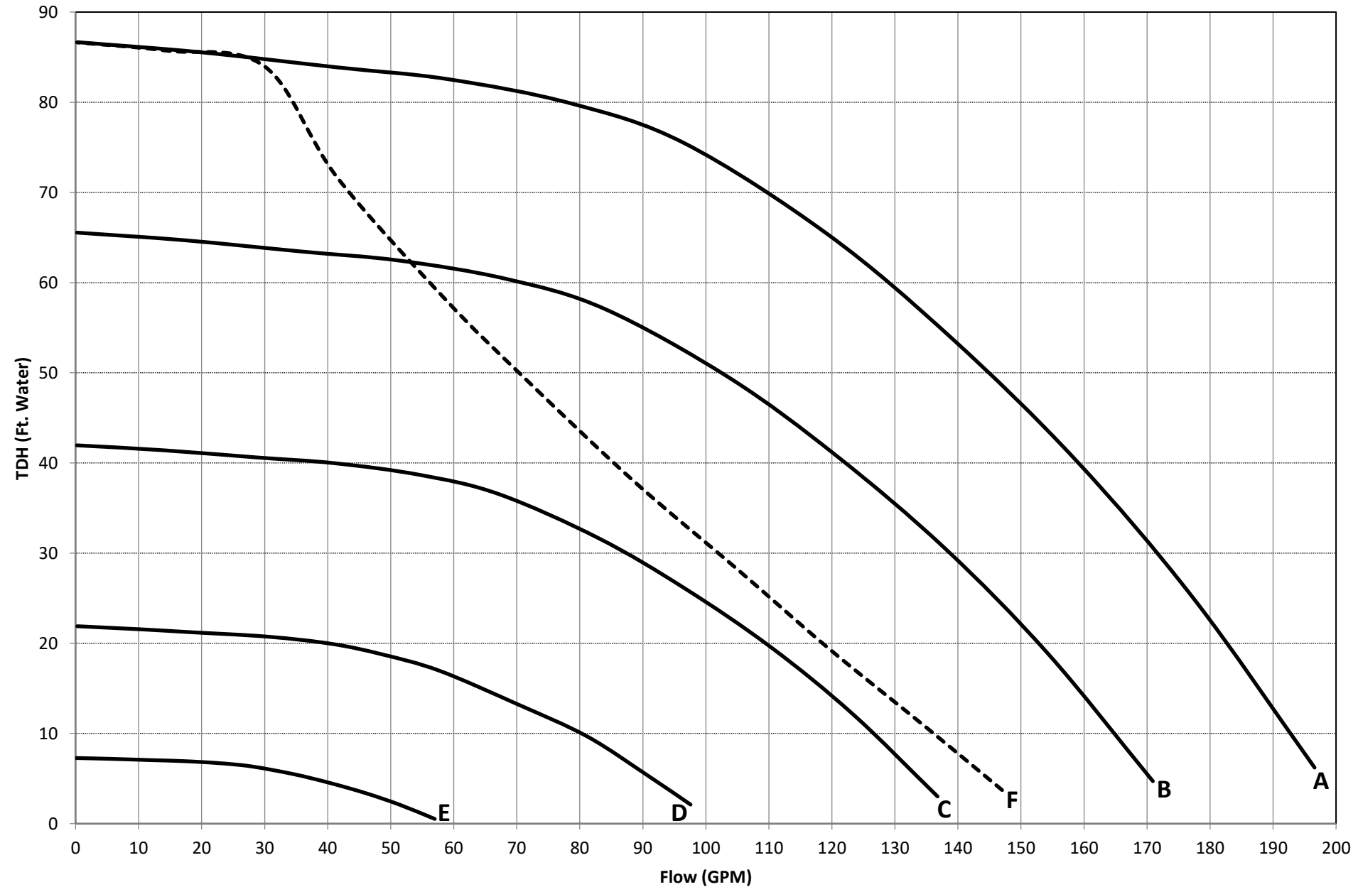
SP32950VSP Performance Curves
