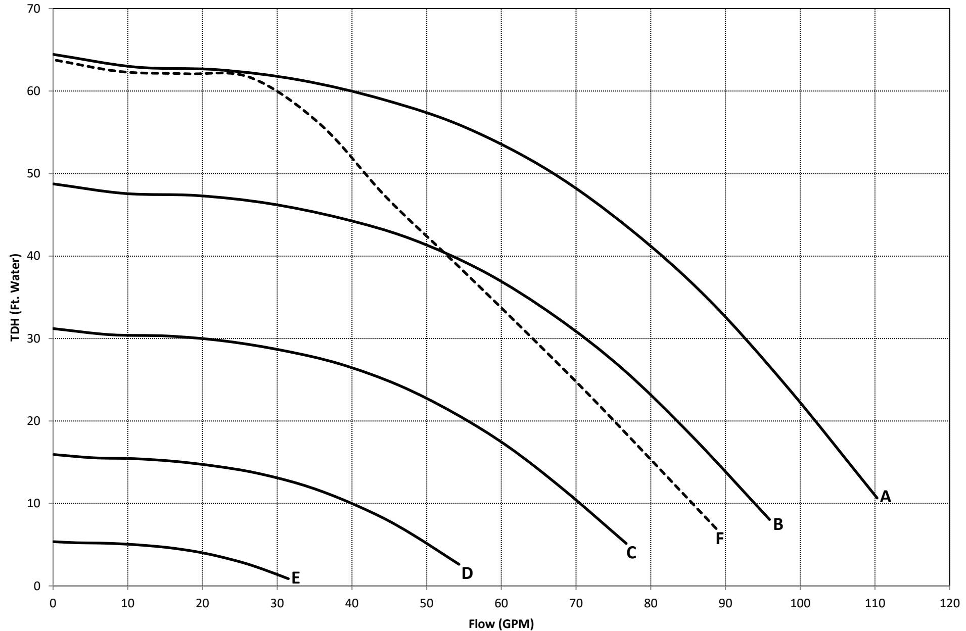
SP2670020VSP Performance Curves
