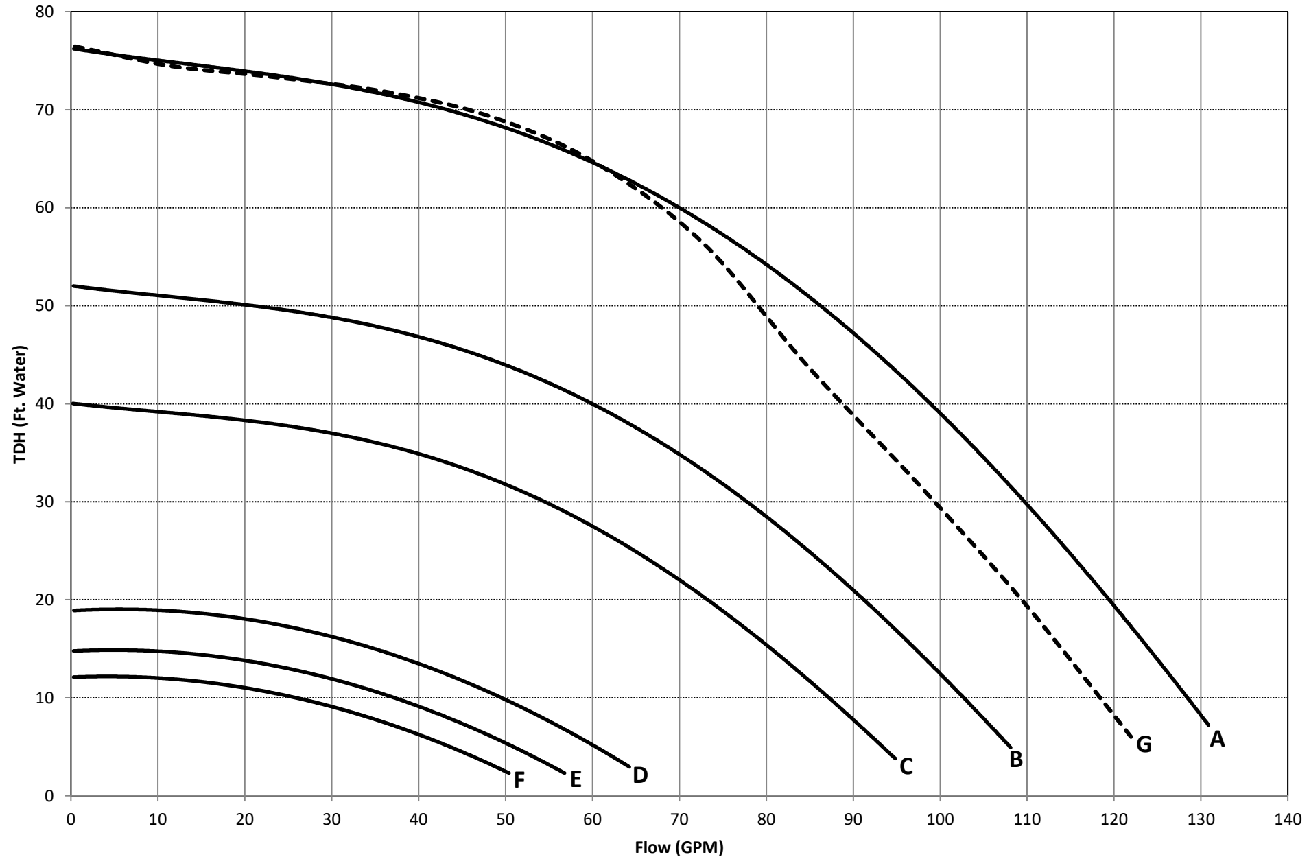
SP2615X20XE Performance Curves
