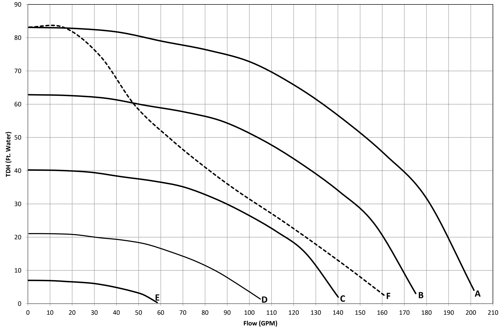
HCP3020VSP Performance Curves
