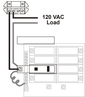
Wiring GFCB for 120 VAC Pool Equipment
